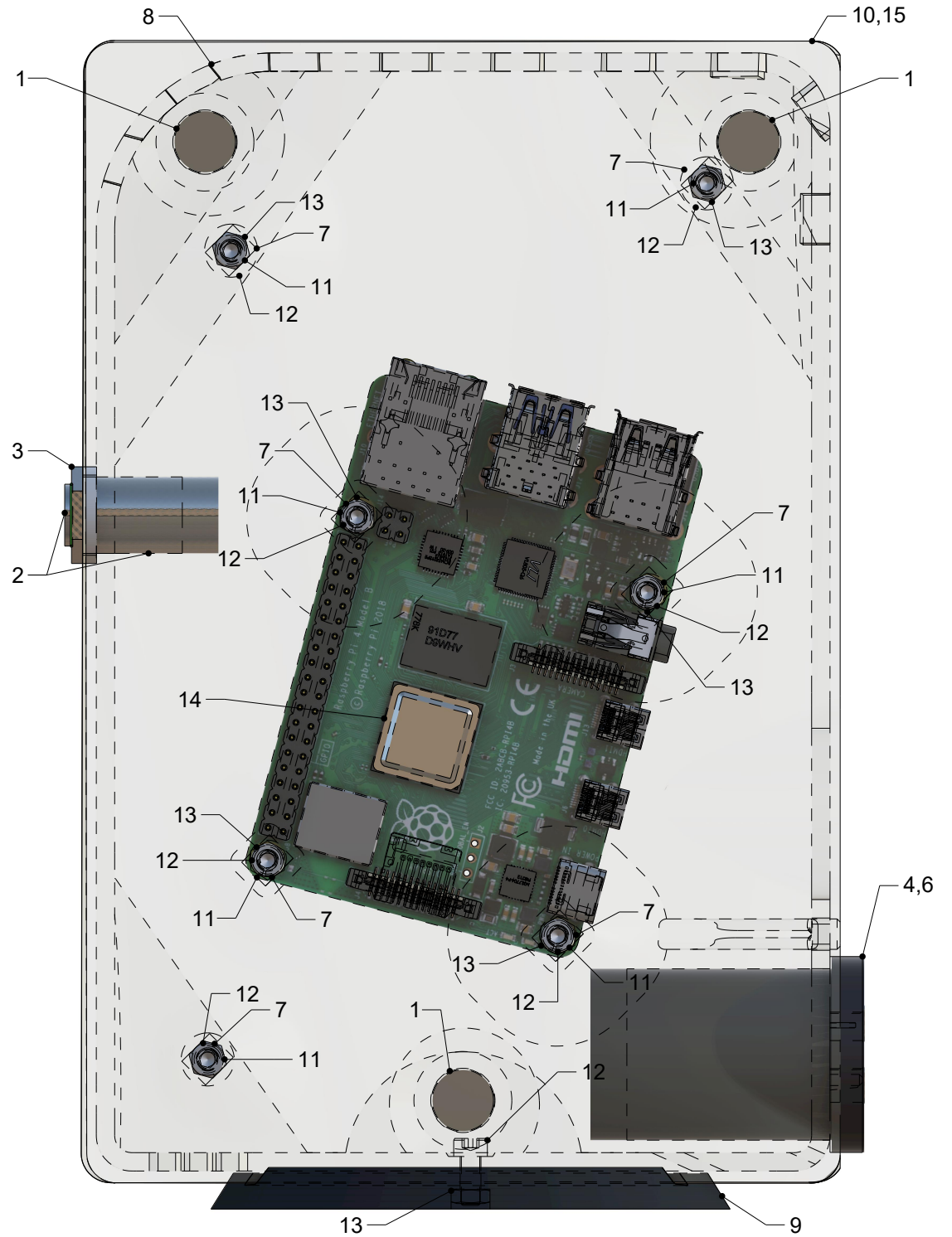
RIGHT VIEW
