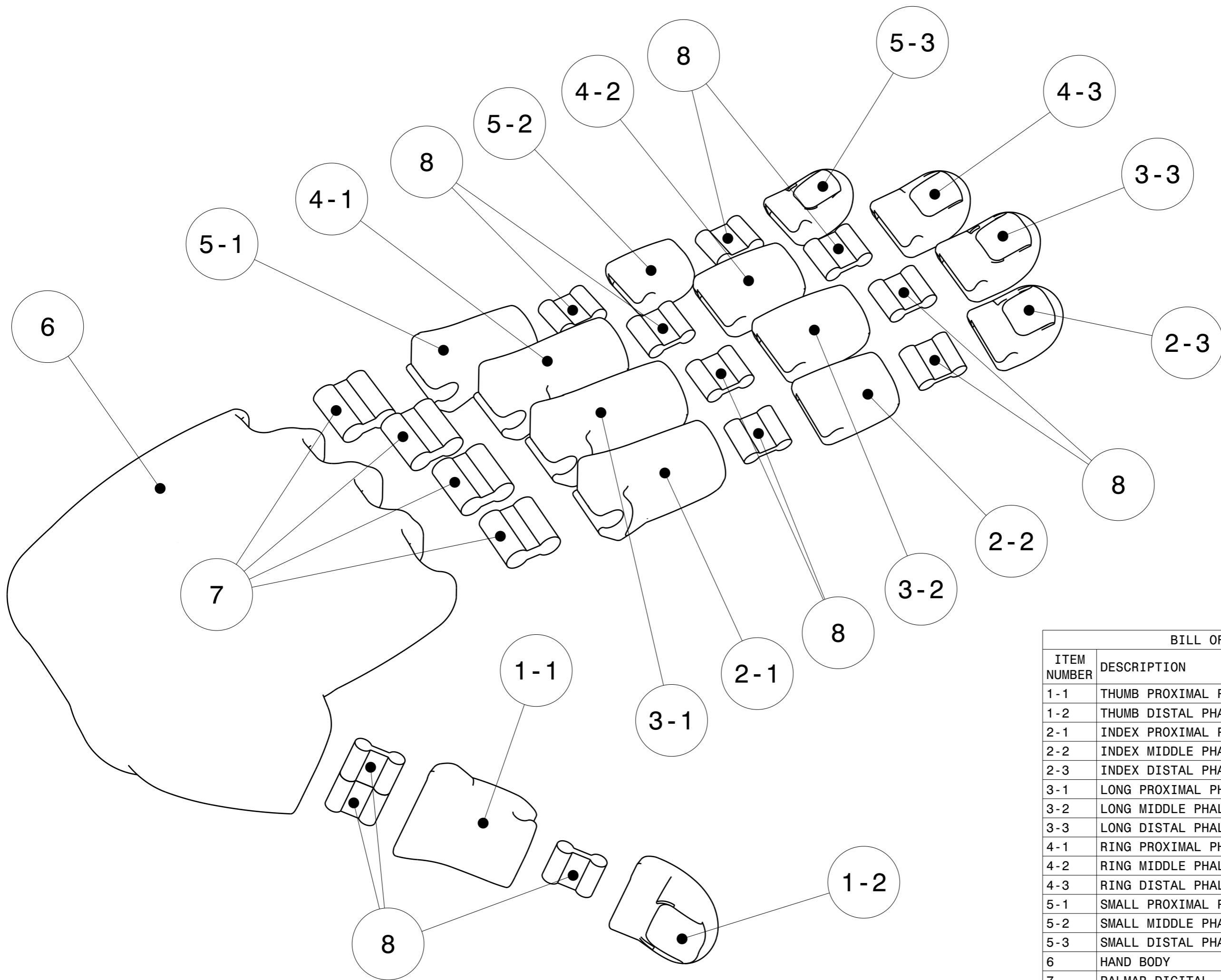
EXPLODED VIEW
